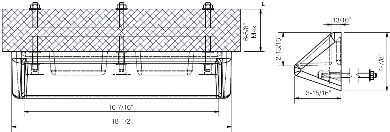
ALF01 - Through Wall Mount
